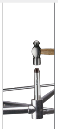
E294 Press-fit Bearing Removal Tool
